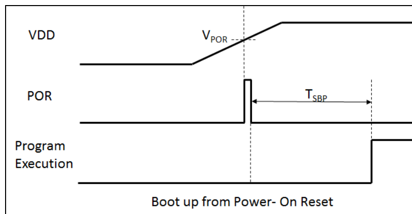
Fig.1: Power-Up Sequence
